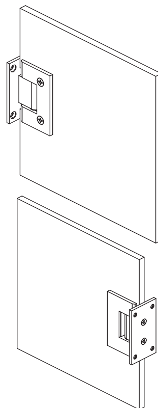
ISO VIEW-3
